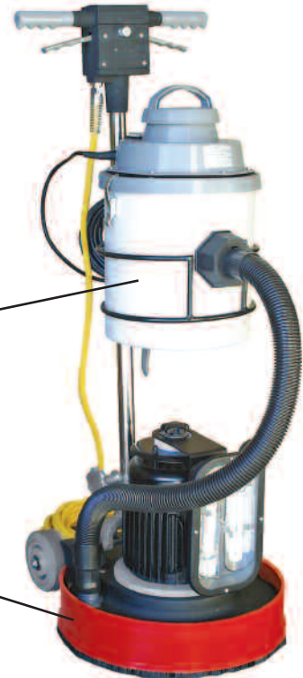
#485-17-VAC-L 17" Extreme Machine with vac ready base, Dust Control Conversion Kit (kit includes pad driver, Dust Control Ring, and light). 7 gal. handle mounted vacuum and hose included.
